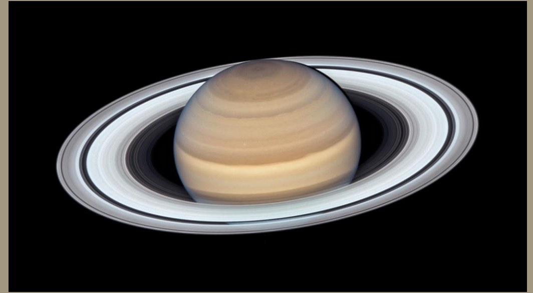
SATURN
