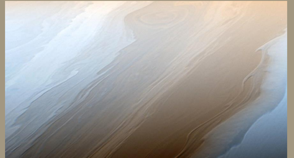
SATURN
